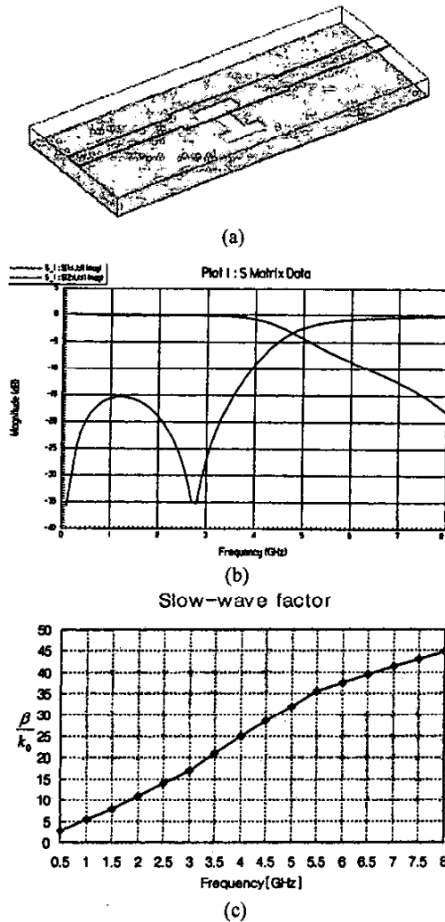
Fig. 1 (a) Schematic of DGS transmission line (b) S_{21} , S_{11} characteristics (c) Slow-wave factor
