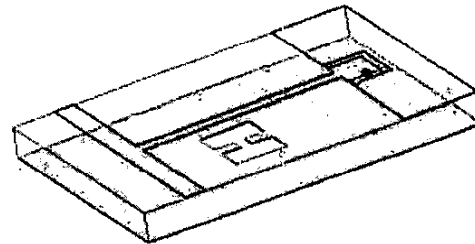
Fig. 2 Layout of DGS \lambda/4 bias transmission line
